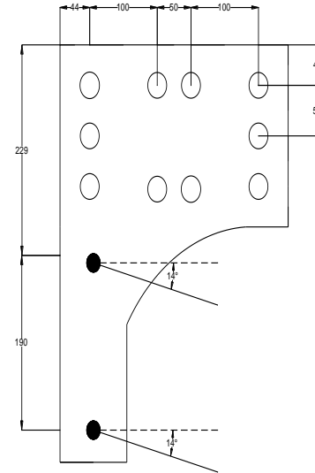
Fig. 2 HANGER BRACKET
