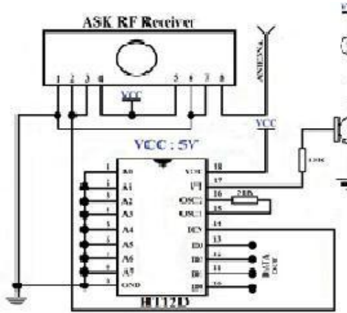
Fig.4 circuit diagram of receiver
