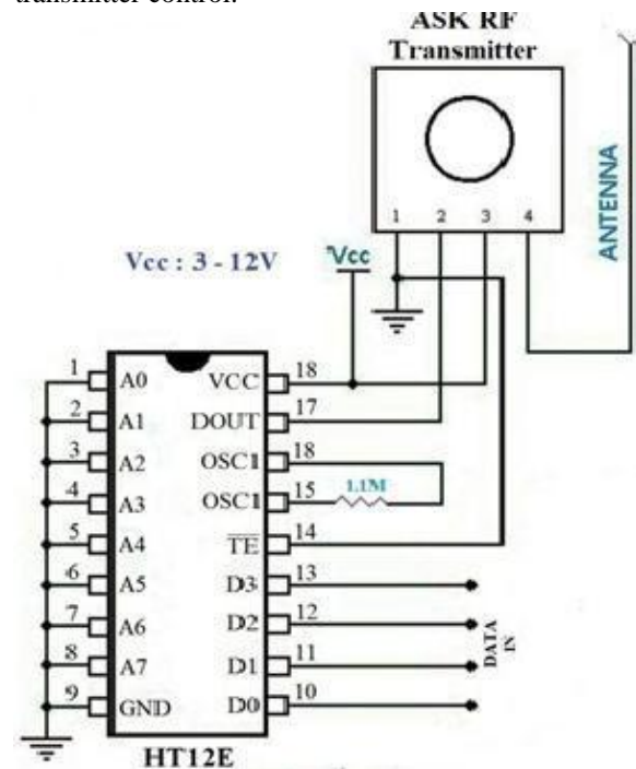
Fig.3 circuit diagram of transmitter
