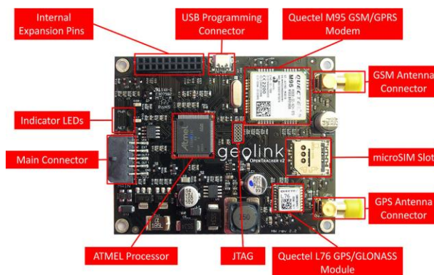
Fig 5. Gateway: Arduino GSM Shield.
