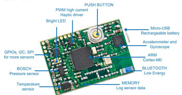
Fig 2. Proposed wearable IoT Device.
